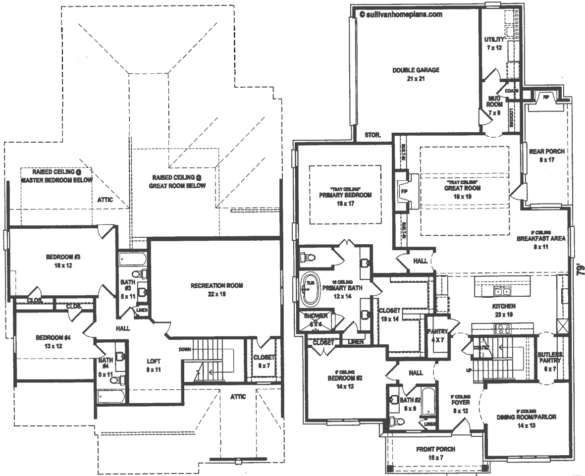
FIRST LEVEL FLOOR PLAN 48'
